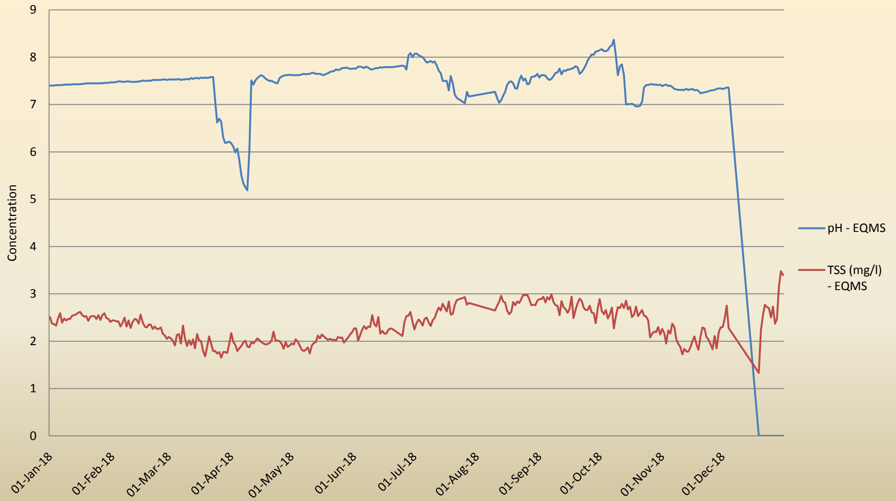
Annual Effluent Trend in M/s. Jaypee Power Ventures Limited, Dist. Singrauli (M.P.)
